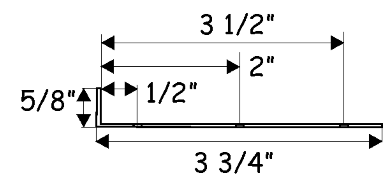
Motor mount dimensions
